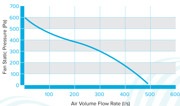
ILMEC 315 PERFORMANCE CURVE
