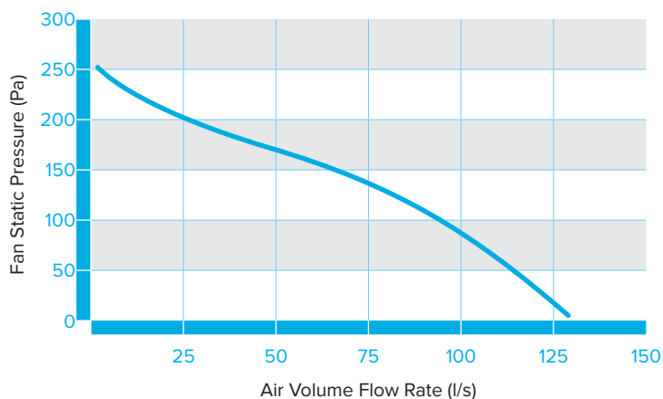
ILMEC 125 PERFORMANCE CURVE
