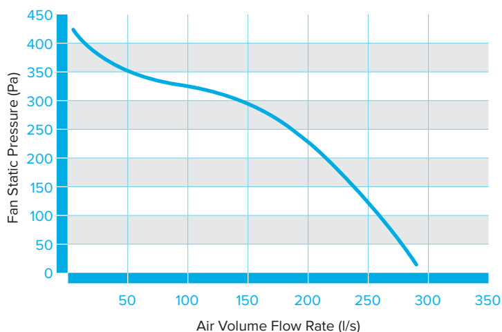
ILMEC 200 PERFORMANCE CURVE
